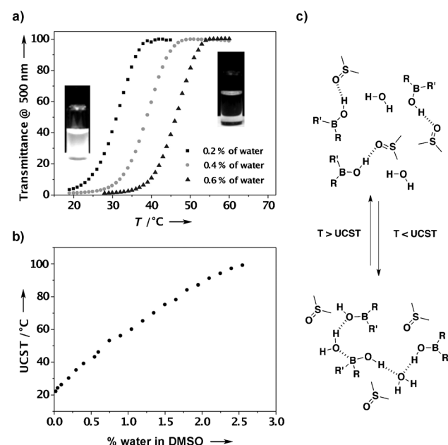
Figure 2. a,b) Plots illustrating the temperature-responsive properties of PBA in DMSO ( 1 \text{ mg mL}^{-1} ) in the presence of different amounts of water (v/v) ( [\text{PBA}] = 1 \text{ mg mL}^{-1} ). The temperature with a transmittance of 50 % is used to determine the UCST. c) Illustration of the proposed mechanism.
